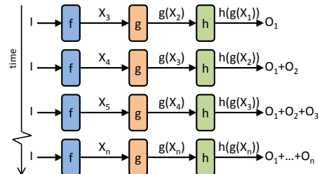
Figure 9: Synchronous pipeline example.
